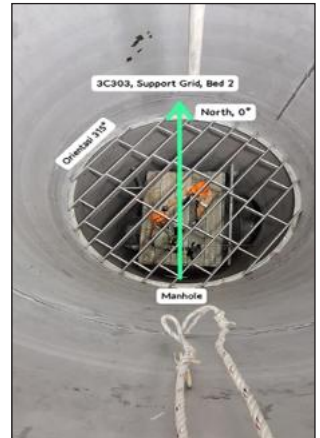
Support grid 3C303
