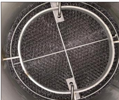
Distributor Installed
