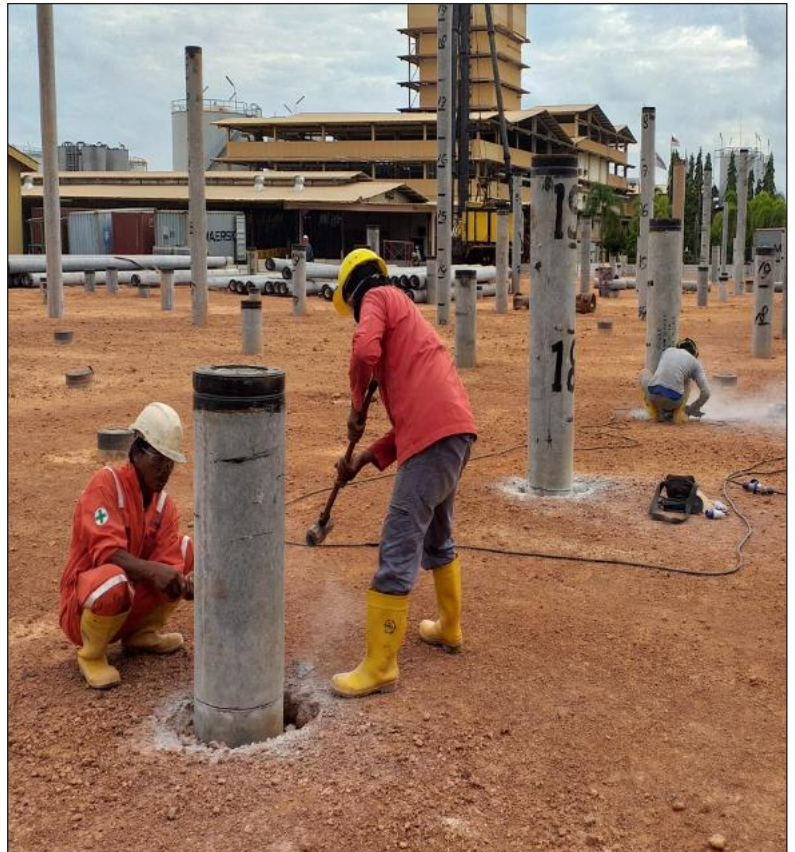
Cutting of Pile
