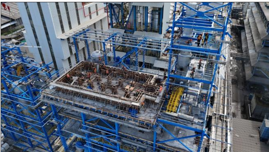
Concrete Pouring Preparation Works
