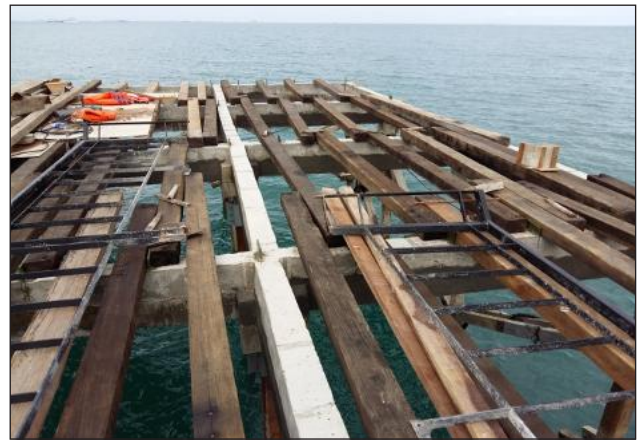
Installation of Timber Joist
