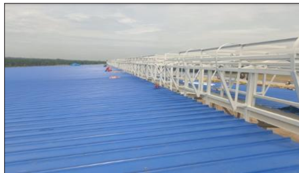
Roof installation works on steel structure
