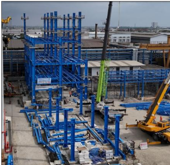
Erection Column Oil Hydrogenation Plant
