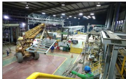
Lifting of Steel Structure
