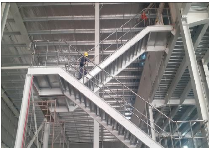
Erection of Internal Staircase for Mezzanine
