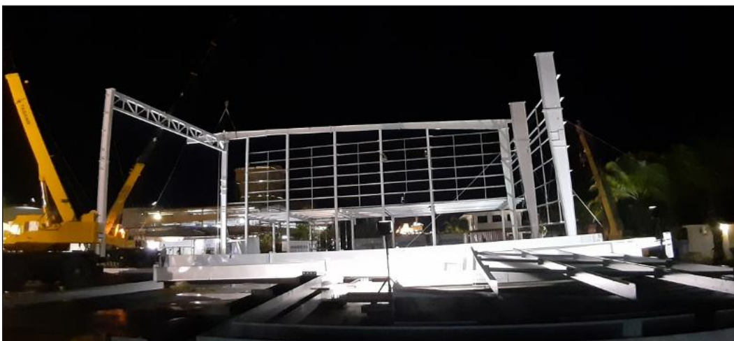
Erection of Truss
