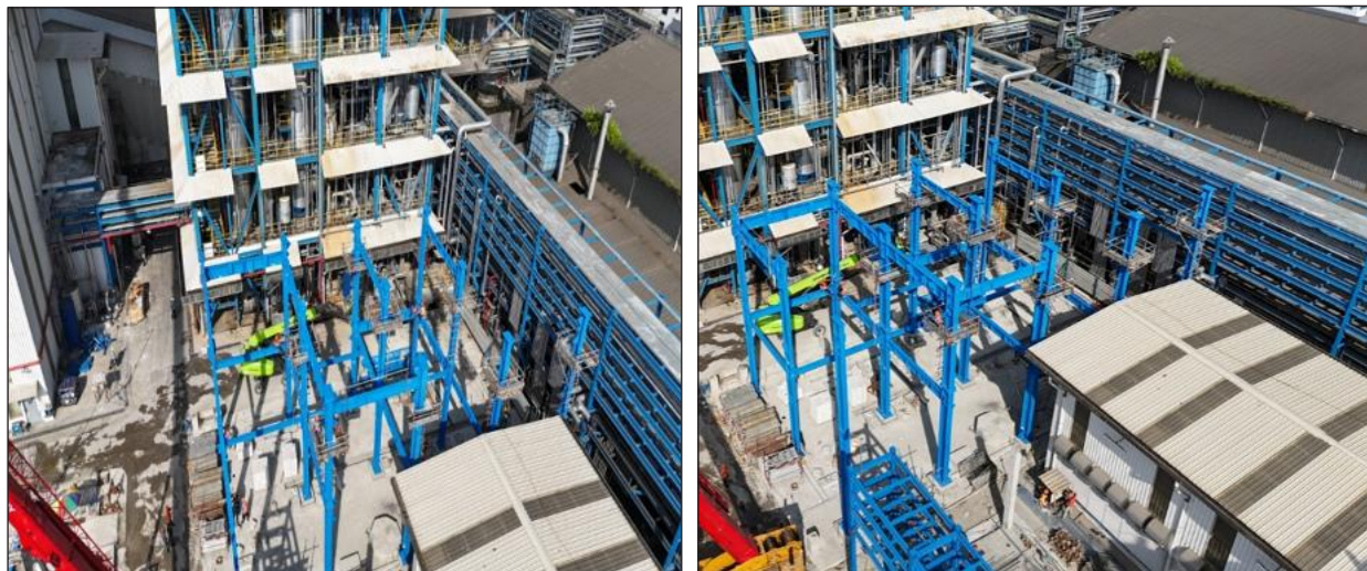
Erection Column Glycerine & Fatty Acid
